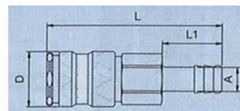
Hose connection
